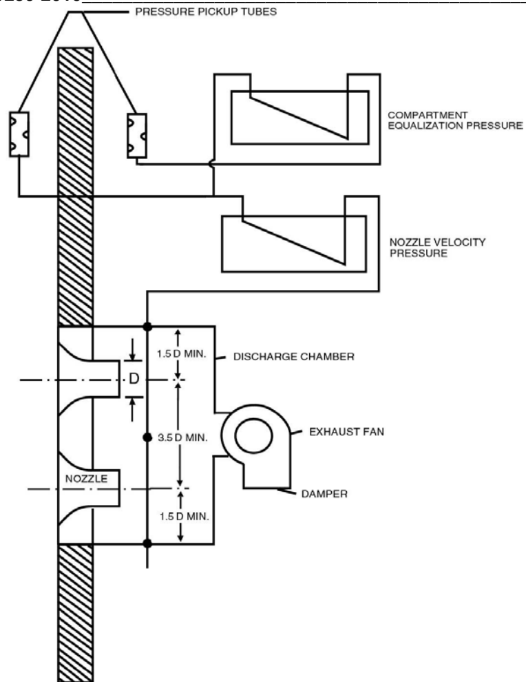
Figure D15. Pressure-Equalizing Device
