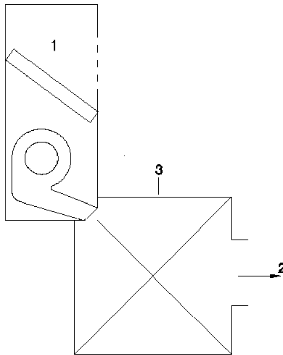
Figure D4. Setup for Wall Mounted Indoor Units 1 – Indoor Unit, 2 – Duct Outlet, 3 – Transition Duct
